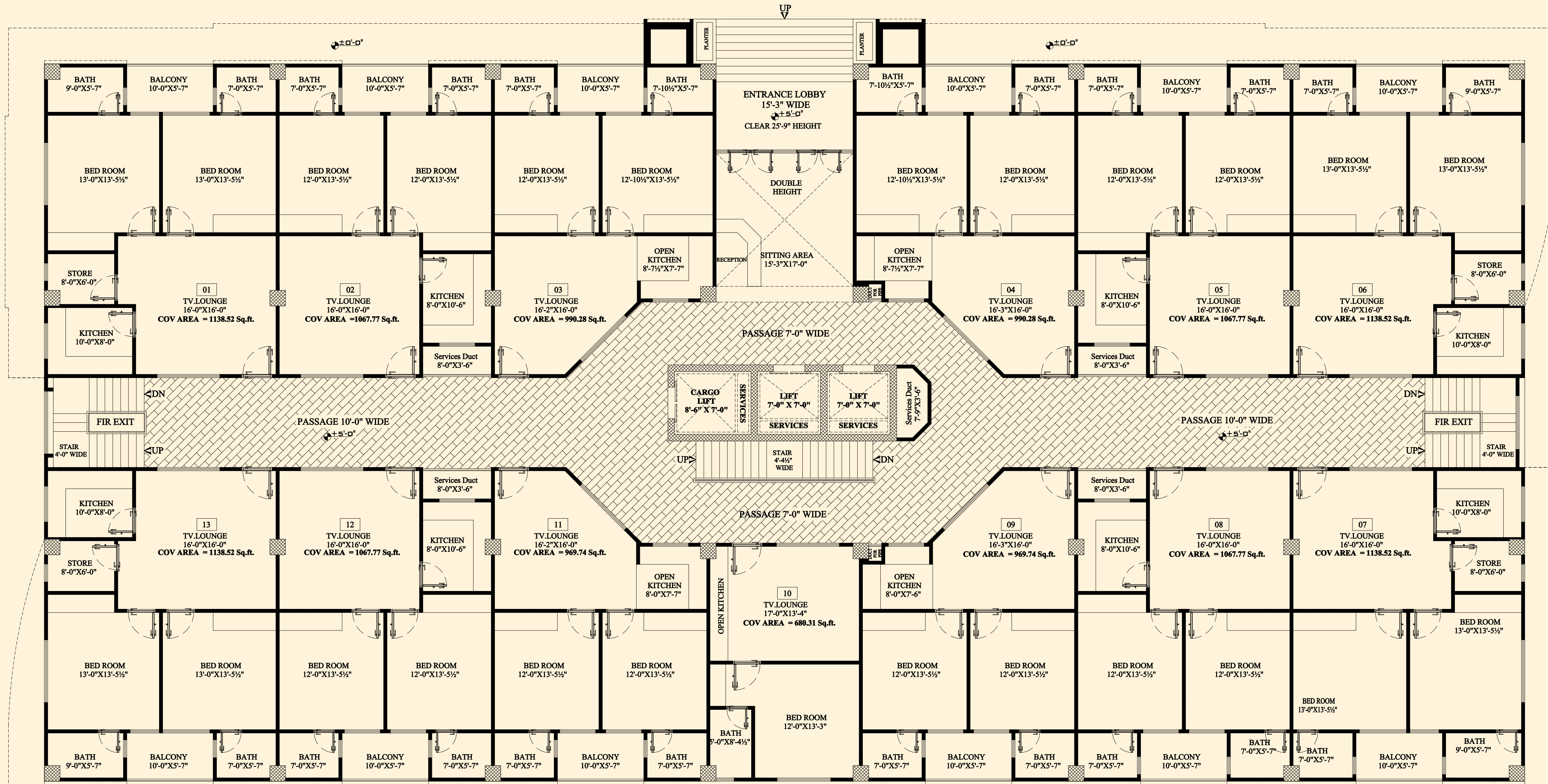
GROUND FLOOR LAYOUT PLAN
